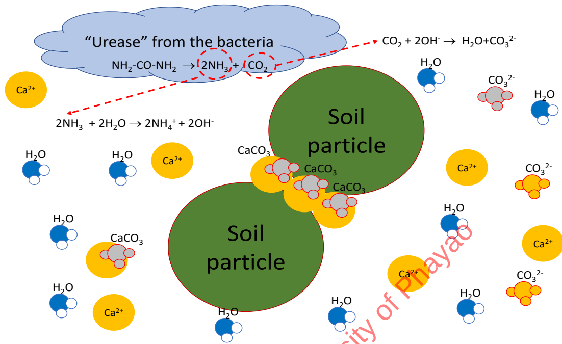
Figure 6-1 Biocementation process via MICP after Petcherdchoo et al. (2026).
