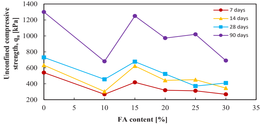
Figure 7-7 Variation of q_u and FA contents of stabilized Bangkok soft clay after Petcherdchoo et al. (2023).
