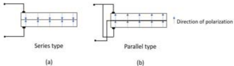
Figure 3-2 (a) Series and (b) Parallel connected bender elements after Iamchaturapatr et al. (2022a).
