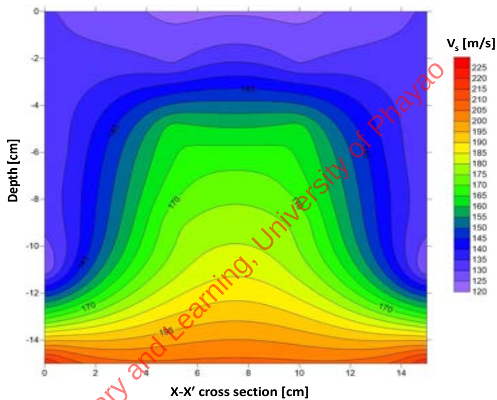
Figure 6-8 Contour of shear wave velocity for sample no.1 at cross section X-X' after Petcherdchoo et al. (2026).
