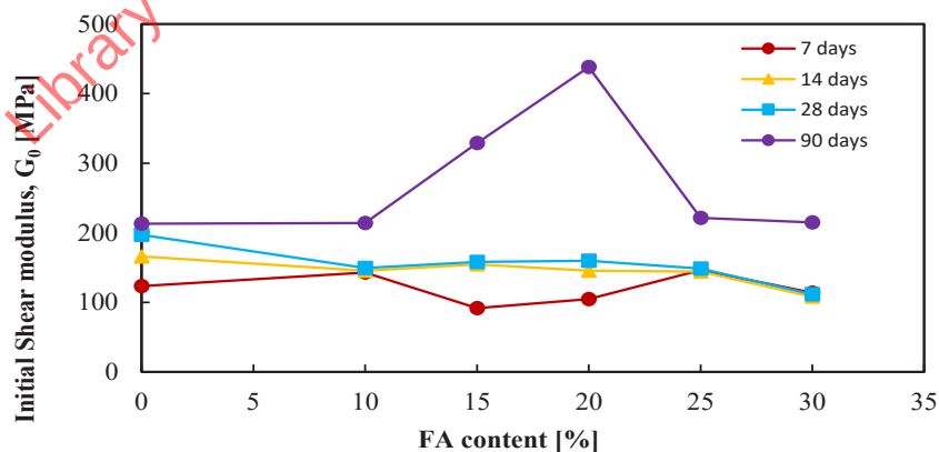
Figure 7-6 Variation of G_0 and FA contents of stabilized Bangkok soft clay after Petcherdchoo et al. (2023).
