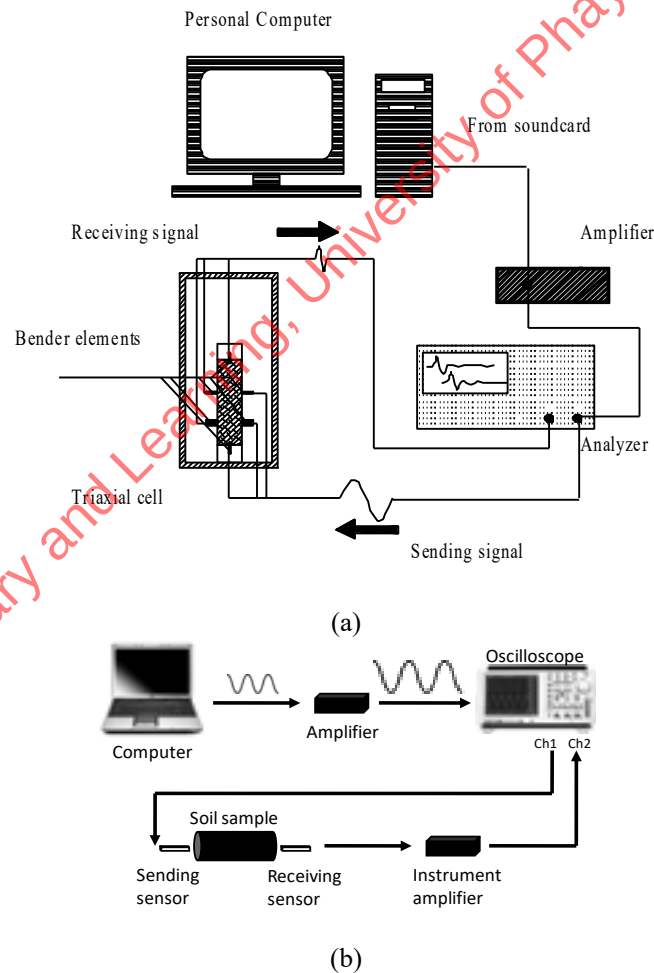
Figure 1-8 a) Bender Element Testing (BET) configuration and b) Schematic diagram after Piriyaikul (2010).
