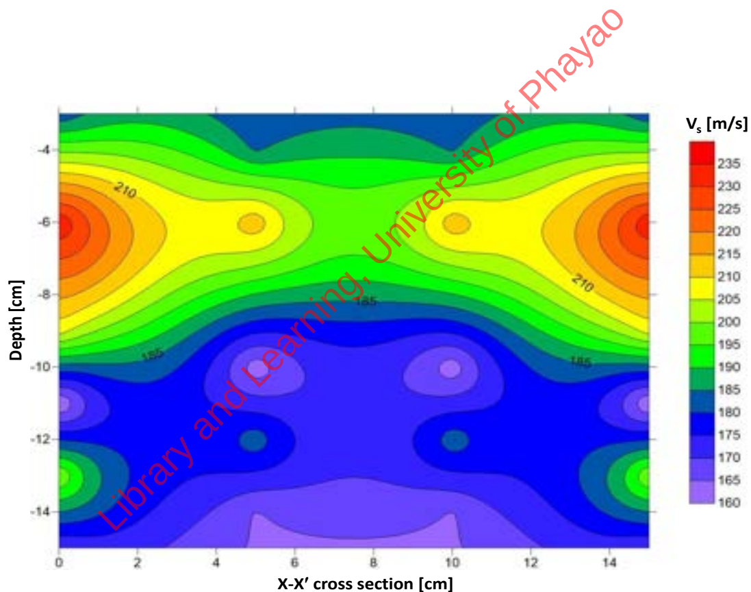
Figure 6-14 Contour of shear wave velocity for sample no.4 at cross section X-X' after Petcherdchoo et al. (2026).
