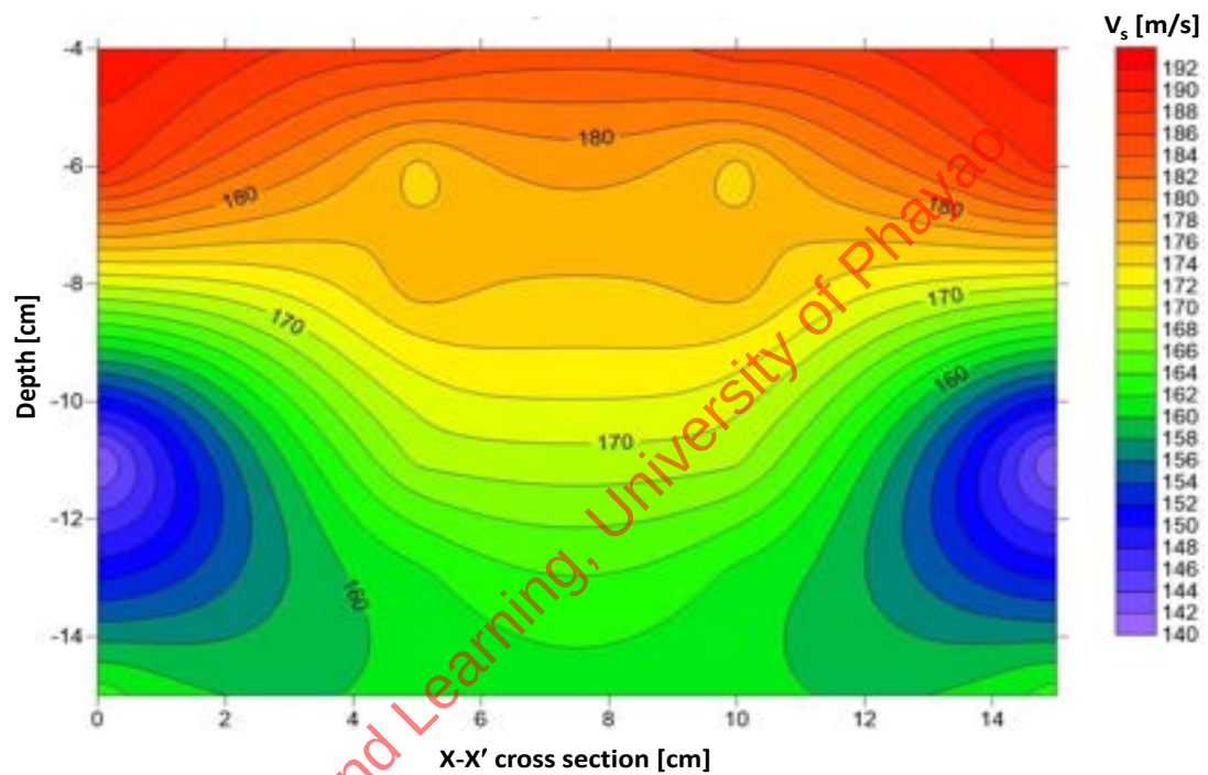
Figure 6-12 Contour of shear wave velocity for sample no.3 at cross section X-X' after Petcherdchoo et al. (2026).
