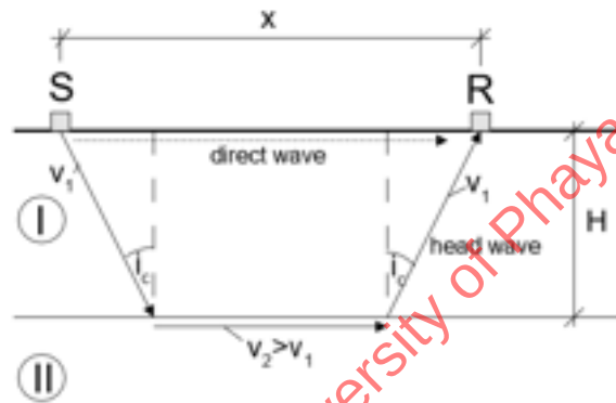
Figure 3-20 Ray paths for the seismic refraction test after Kramer (1996).
