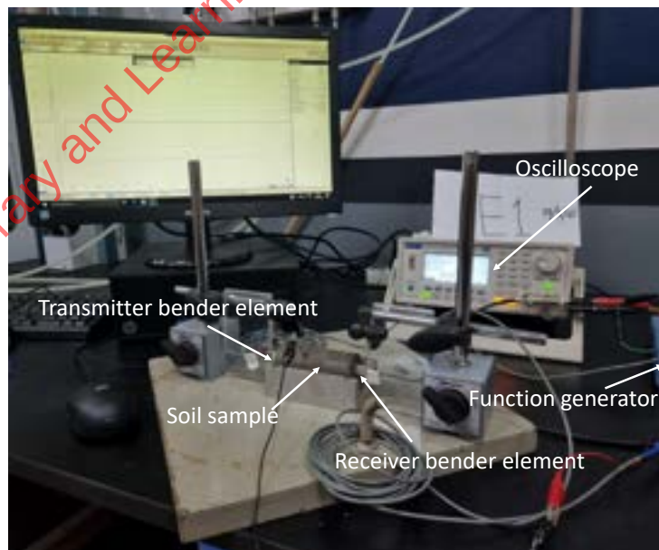
Figure 3-6 Bender element test setup at the KMUTNB campus.
