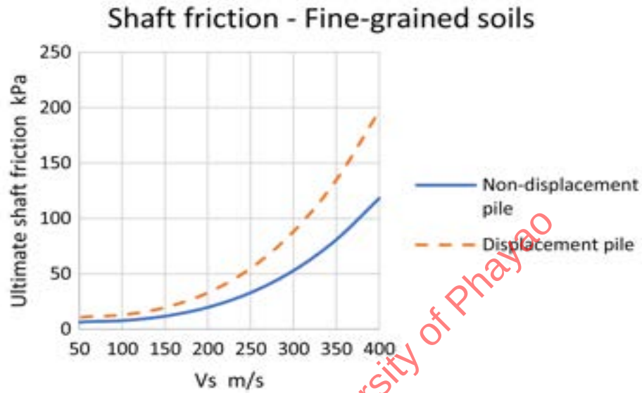
Figure 3-28 Ultimate shaft friction versus V_s for fine-grained soils after Poulos (2022).
