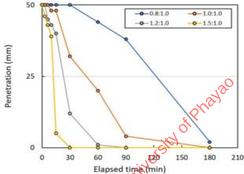
Figure 5-9. The penetration varied with elapsed time for the mixing proportion between the metakaolin treated at 800°C and the geopolymer solution after Iamchaturapatr et al. (2022b).
