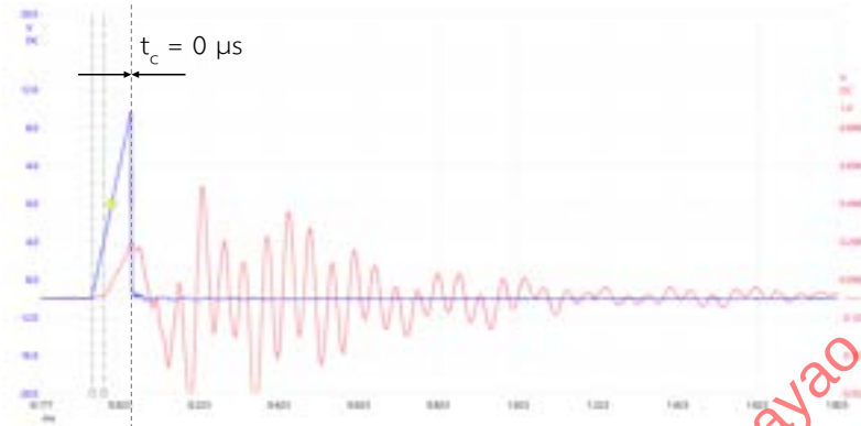
Figure 4-34 Measurement of calibration time for 1 triangle signal.
