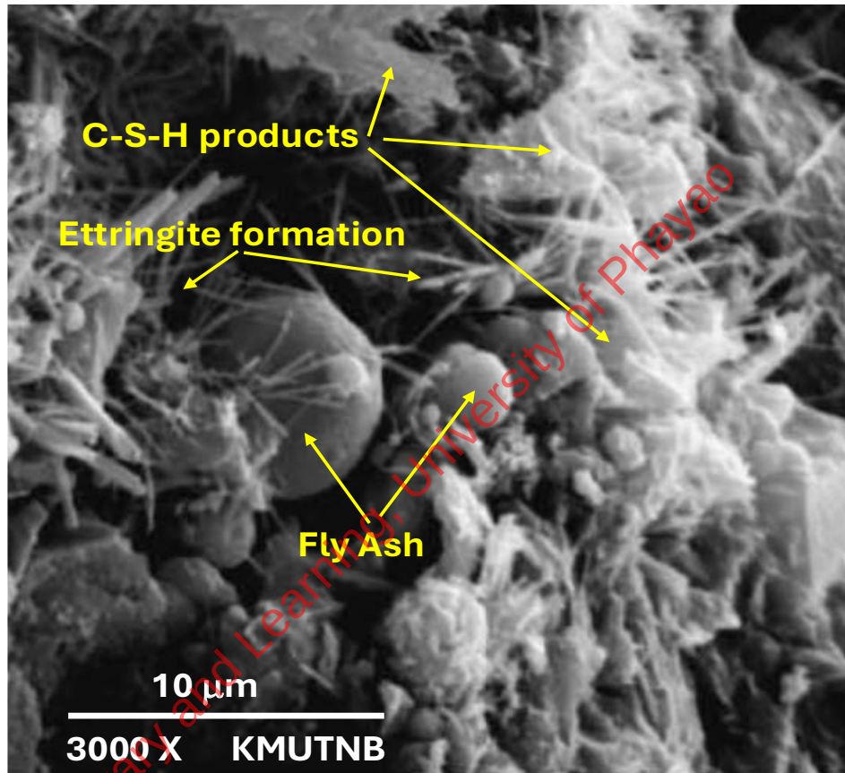
Figure 7-11 SEM image of 20% FA sample at 28 days after Petcherdchoo et al. (2023).
