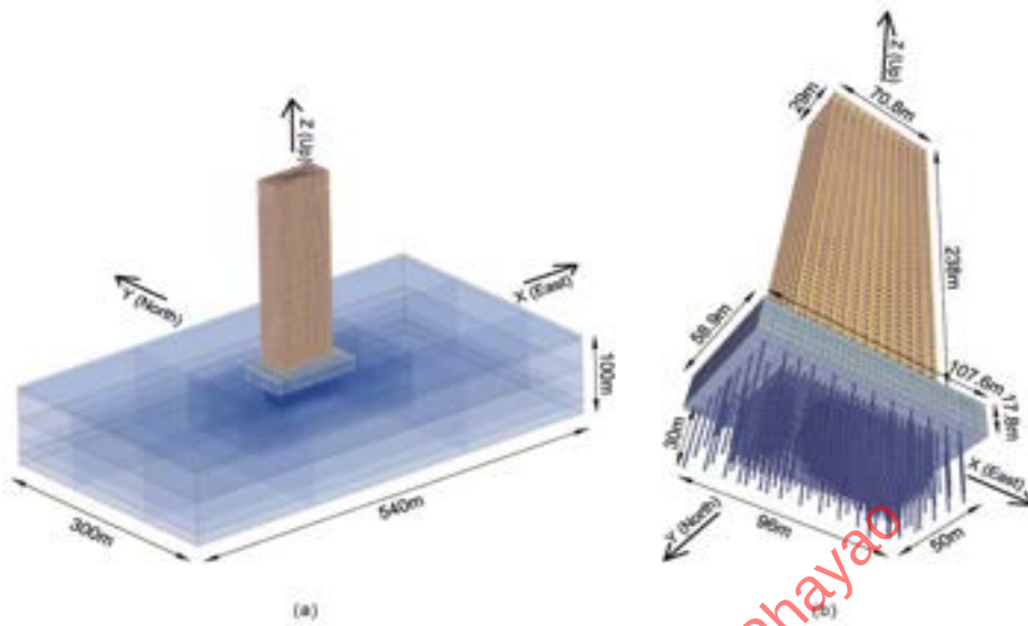
Figure 3-28 FEM model a) a complete model and b) foundation after Cruz et al. (2024).
