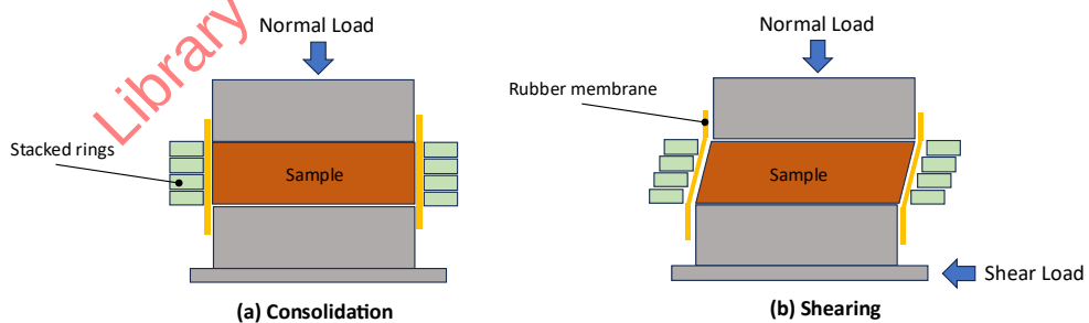
Figure 3-10 (a) Consolidation phase and (b) Shearing phase.
