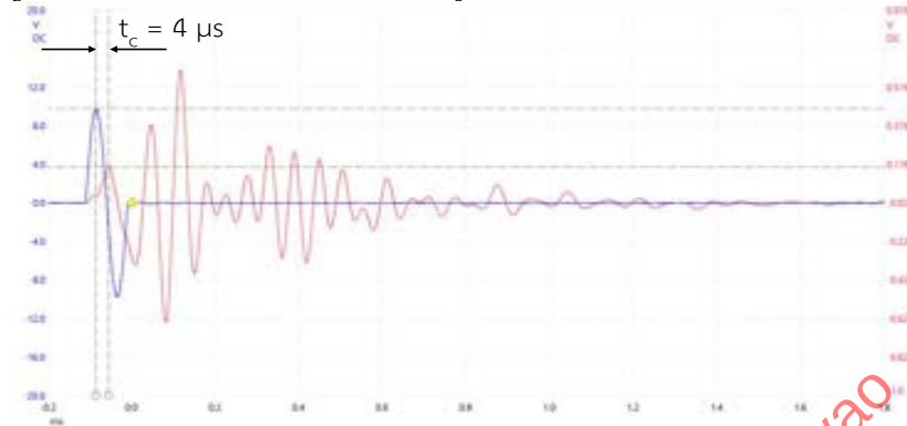
Figure 4-30 Measurement of calibration time for 1 sinusoidal signal.
