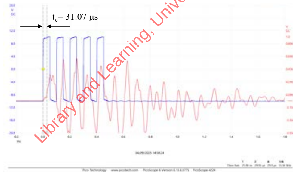
Figure 4-10 Calibration of bender element with a 5-period rectangle waveform.
