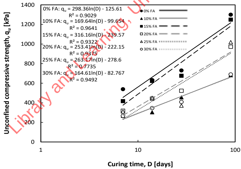
Figure 7-4 Development of q_u with curing time of FA stabilized Bangkok soft clay after Petcherdchoo et al. (2023).
