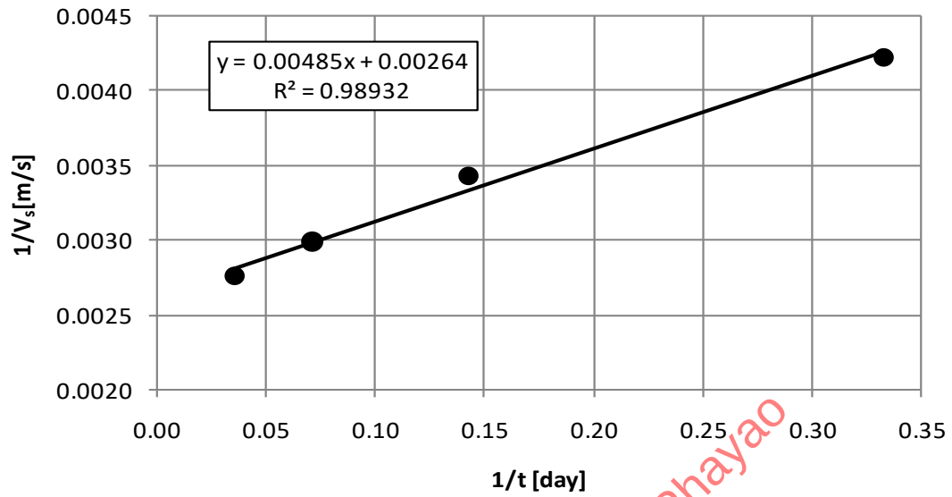
Figure 4-25 The relationship between \frac{1}{V_s} and \frac{1}{t} after Piriyaikul (2013b).
