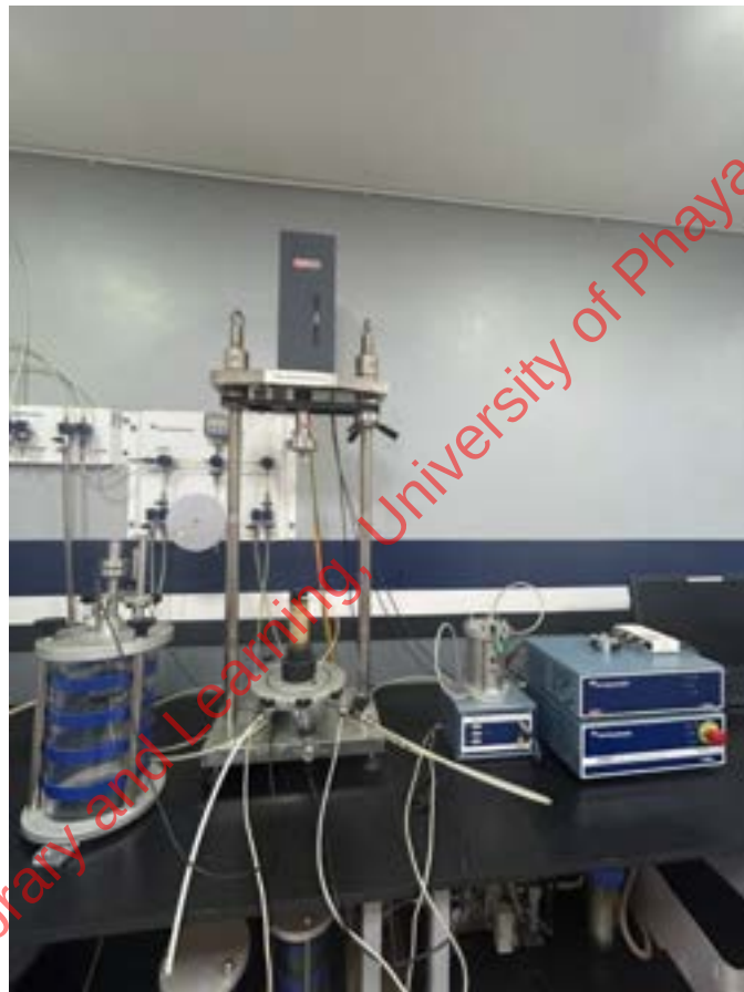
Figure 3-7 Cyclic triaxial test at the KMUTNB campus.
