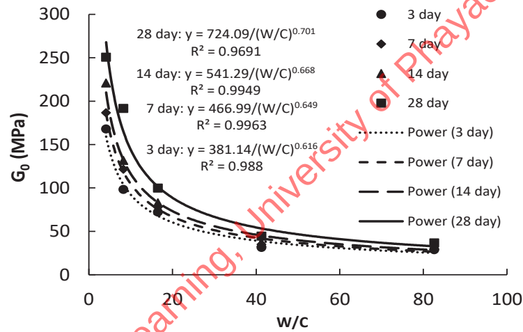
Figure 8-13 G_0 vs W/C after Piriyaikul et al. (2026).
