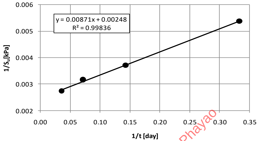
Figure 4-27 The relationship between \frac{1}{S_u} and \frac{1}{t} after Piriyaikul (2013b).
