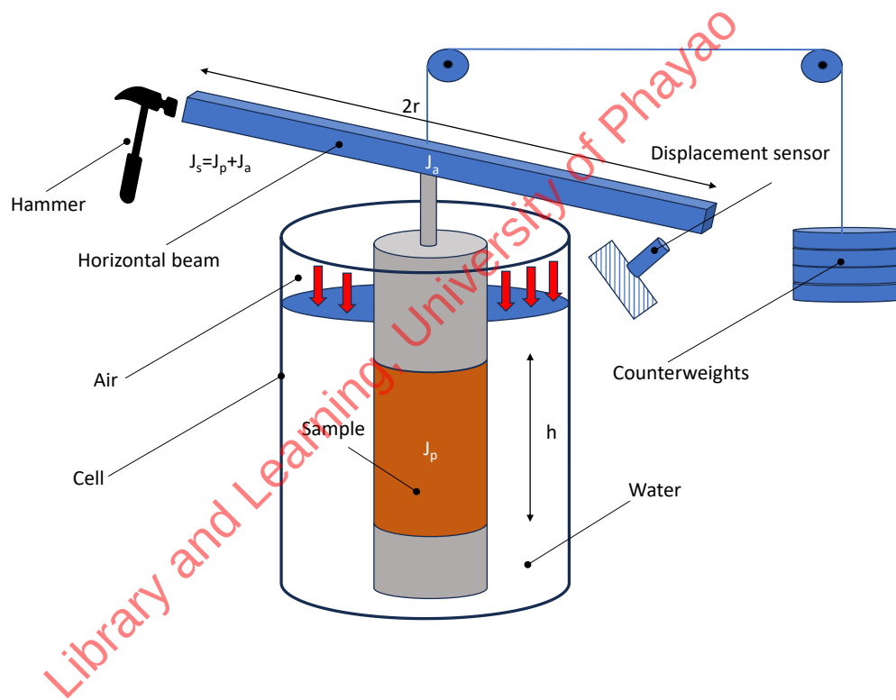
Figure 3-12 Schematic of the free torsion pendulum test after Karl (2005).
