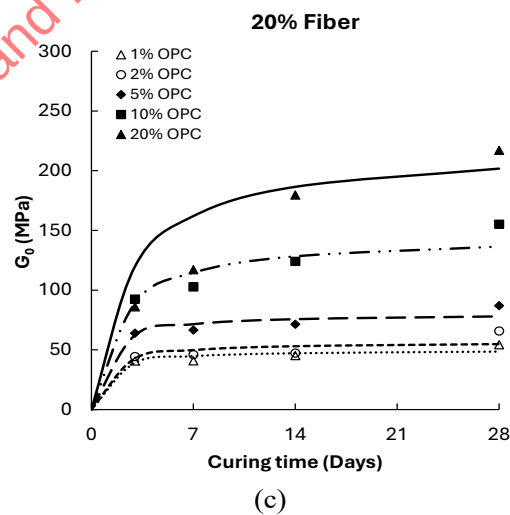
Figure 8-9 G_0 vs Curing time (a) 0% fiber (b) 1% fiber and (c) 20% fiber after Piriyaikul et al. (2026).
