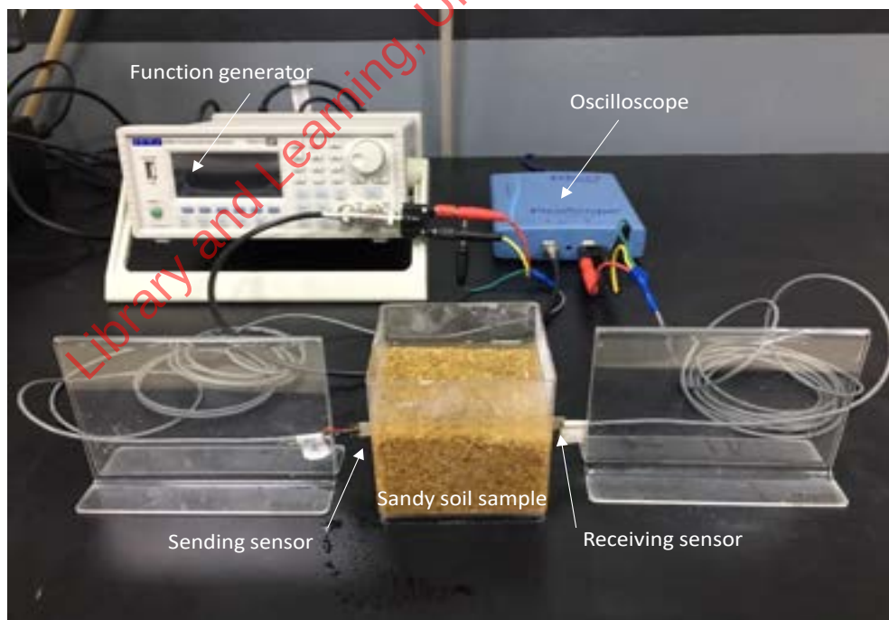
Figure 6-4 Setting-up of bender element testing for BSR after Petcherdchoo et al. (2026).
