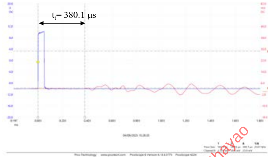
Figure 4-15 Measurement of shear velocity with a single period rectangle waveform.
