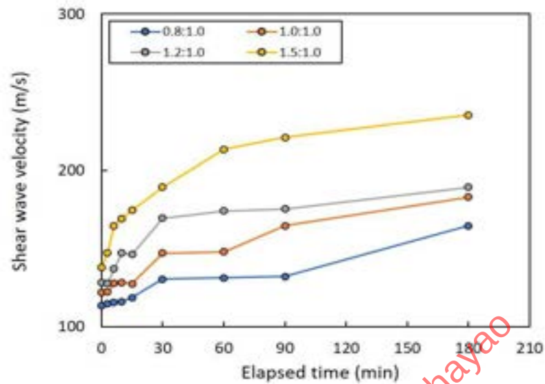
Figure 5-7. The shear wave velocity varied with elapsed time for the mixing proportion between the metakaolin treated at 800°C and the geopolymer solution after Iamchaturapatr et al. (2022b).
