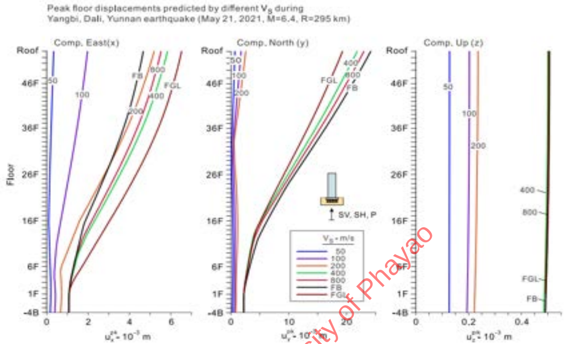
Figure 3-32 Peak floor displacements for different values of V_s during Yangbi, Dali earthquake after Cruz et al. (2024).
