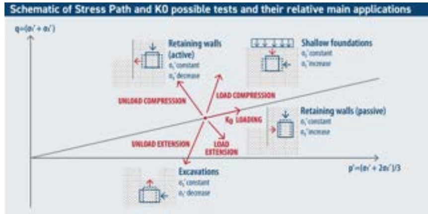
Figure 3-15 K_0 consolidation and shearing in stress path triaxial test after Controls Group (2025).
