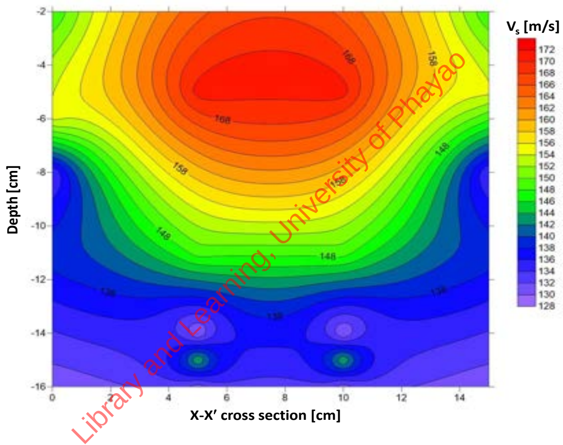
Figure 6-10 Contour of shear wave velocity for sample no.2 at cross section X-X' after Petcherdchoo et al. (2026).
