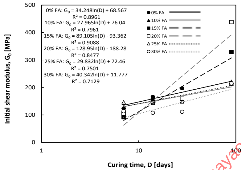
Figure 7-3 Development of G_0 with curing time of FA stabilized Bangkok soft clay after Petcherdchoo et al. (2023).
