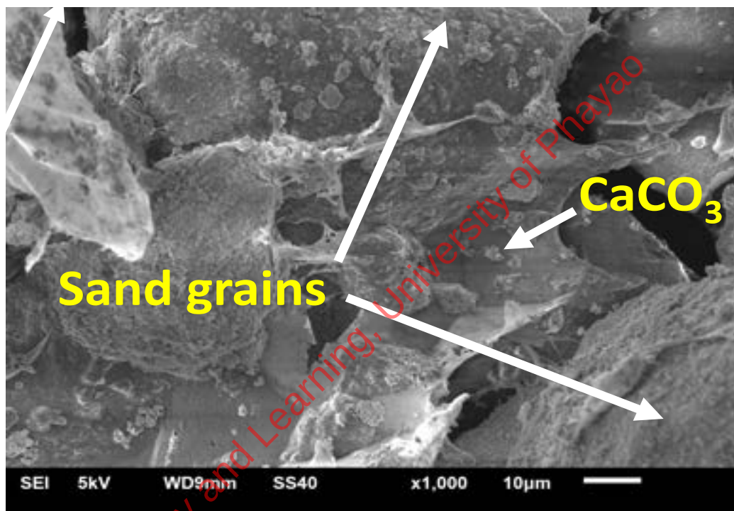
Figure 6-18 SEM image of the biocemented sandy soil at 1000x after Petcherdchoo et al. (2026).
