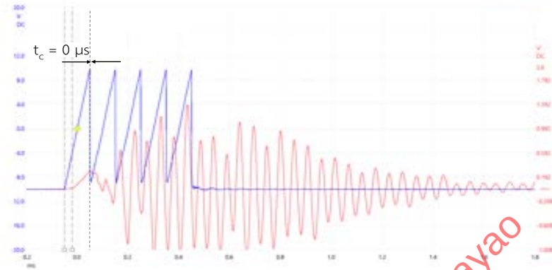
Figure 4-36 Measurement of calibration time for 5 triangle signal.
