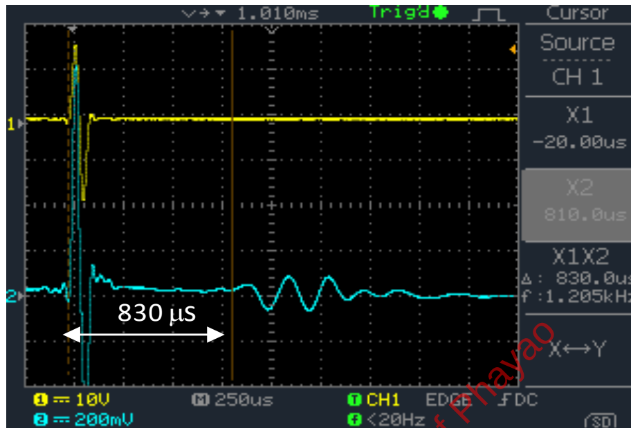
Figure 4-21 Measurement of shear wave velocity of Bangkok clay at 4.0 m depth (Frequency=12,000 Hz) after Piriyaikul (2013a).
