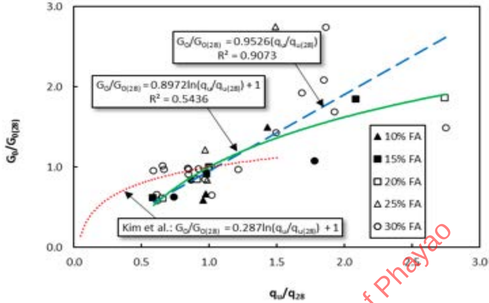
Figure 7-9 Relationships between G_0/G_{0(28)} and q_u/q_{u(28)} after Petcherdchoo et al. (2023).
