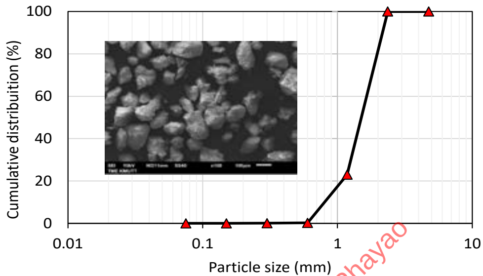
Figure 6-2 Particle size distribution of sandy soils after Petcherdchoo et al. (2026).
