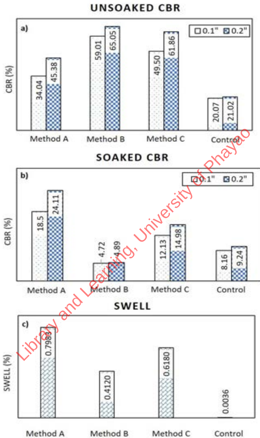
Figure 5-12 CBR test results for different mixing methods and conditions: (a) unsoaked (b) soaked (c) swelling after Iamchaturapatr et al. (2022b).
