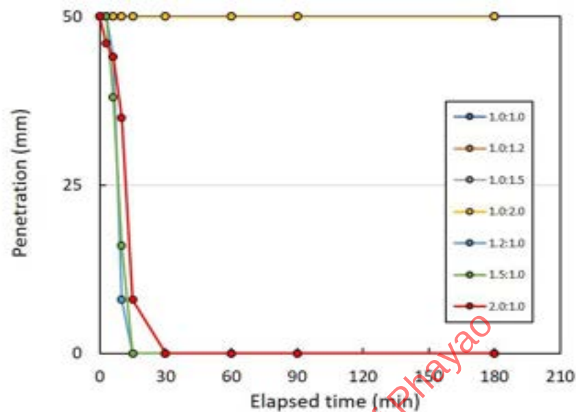
Figure 5-6 The penetration varied with elapsed time for the mixing of geopolymer solution after Iamchaturapati et al. (2022b).
