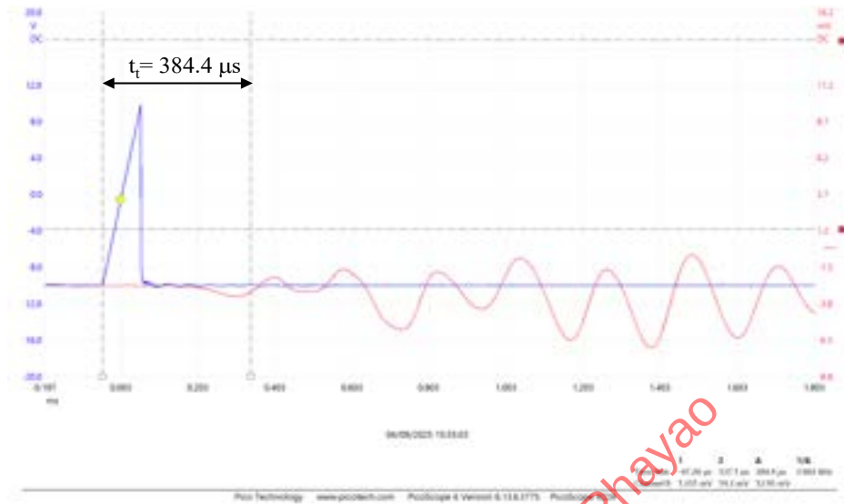
Figure 4-13 Measurement of shear velocity with a single period triangle waveform.
