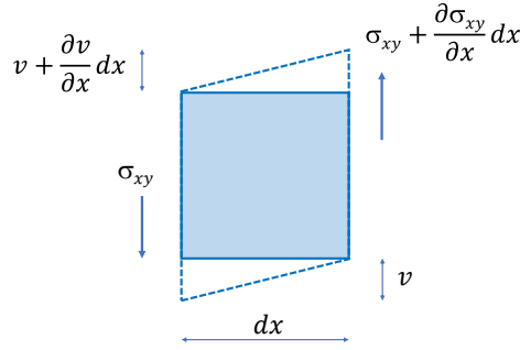
Figure 2-4 Differential stress elements for simple shear stress.
