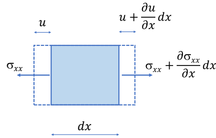
Figure 2-3 Differential stress elements for simple longitudinal stress.
