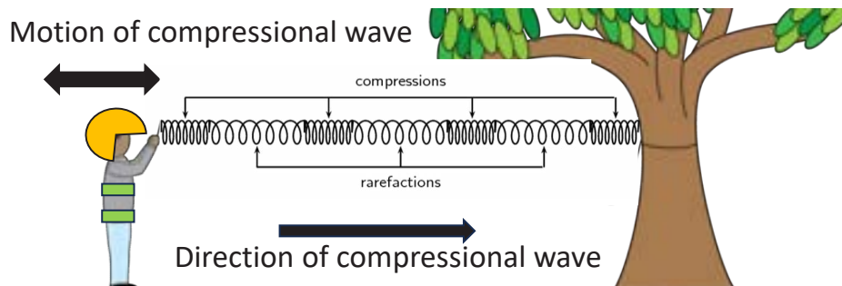
Figure 2-2 Motion of compressional wave (P-wave).
