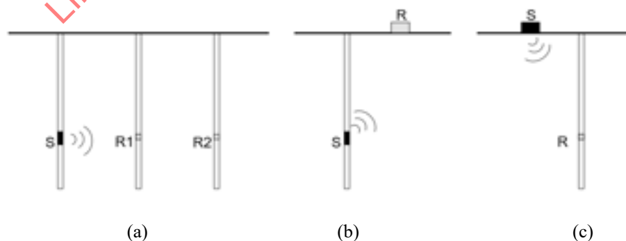
Figure 3-19 (a) Seismic cross-hole test, (b) seismic up-hole test and (c) seismic downhole test after Mok et al. (1988).
