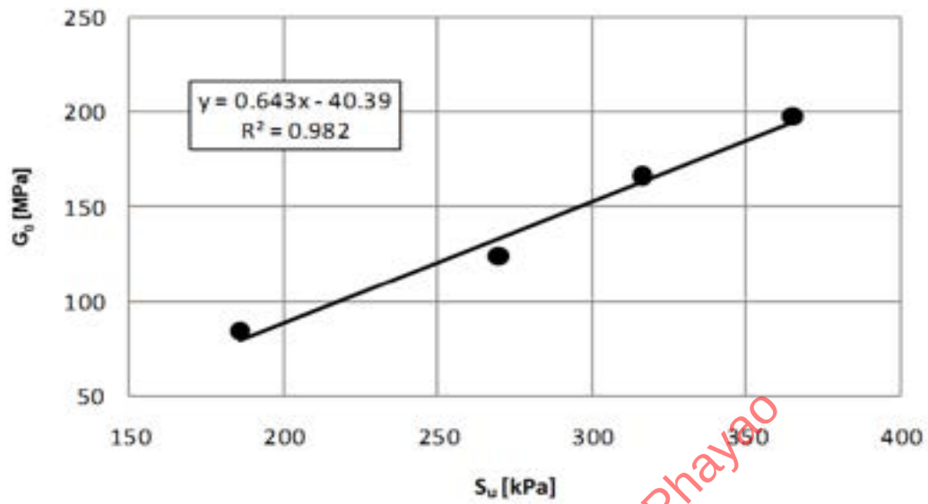
Figure 4-29 The relationship between G_0 and S_u after Piriyaikul (2013b).
