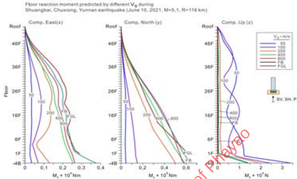
Figure 3-36 Floor moments for different values of V_s during Shuangbai, Chuxiong earthquake after Cruz et al. (2024).
