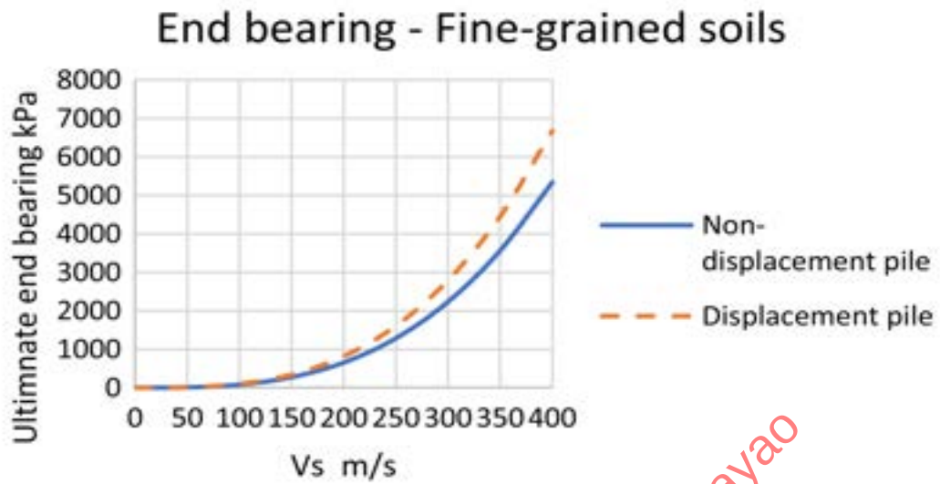
Figure 3-30 Ultimate end bearing versus V_s for fine-grained soils after Poulos (2022).
