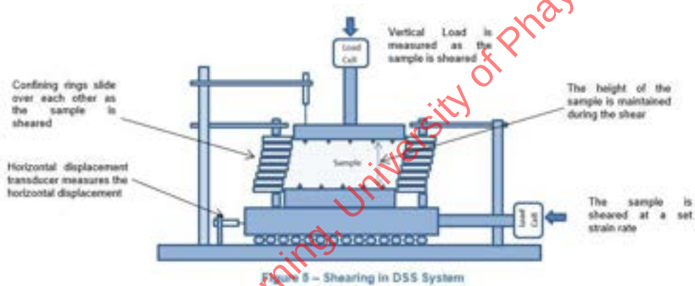
Figure 3-9 Schematic of cyclic simple shear apparatus after VJ Tech (2025).
