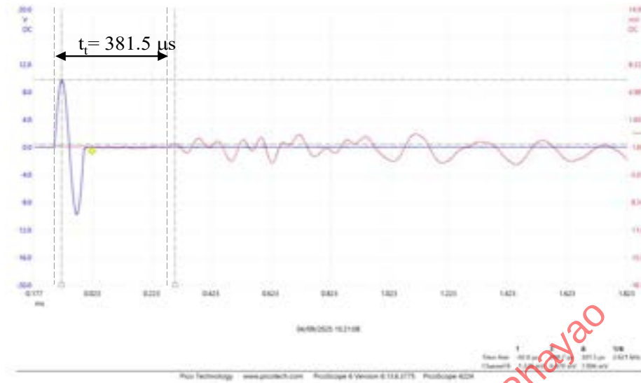
Figure 4-11 Measurement of shear velocity with a single period sinusoidal waveform.
