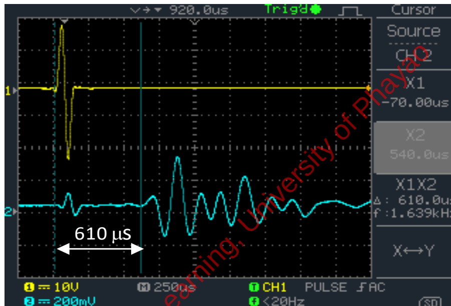
Figure 4-22 Measurement of shear wave velocity of Bangkok clay at 5.0 m depth (Frequency=12,000 Hz) after Piriyaikul (2013a).
