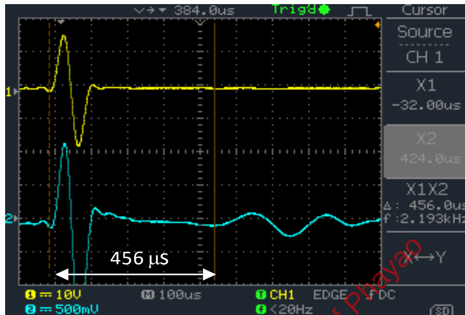
Figure 4-23 Measurement of shear wave velocity of Bangkok clay at 13.0 m depth (Frequency=12,000 Hz) after Piriyakul (2013a).
