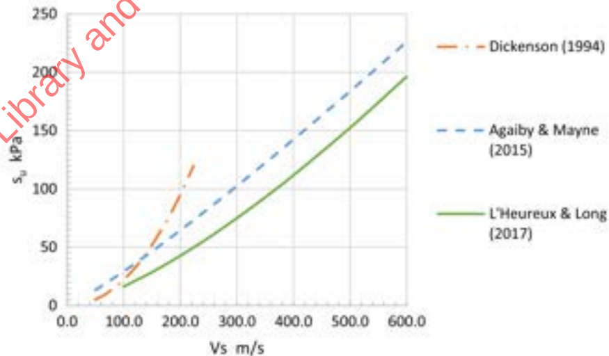
Figure 3-25 Correlations of S_u versus V_s after Poulos (2022).
