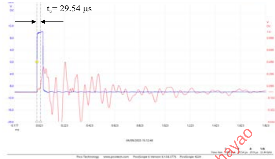
Figure 4-9 Calibration of bender element with a single period rectangle waveform.
