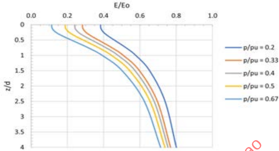
Figure 3-26 Young modulus reduction factors for a shallow circular footing after Poulos (2022).
