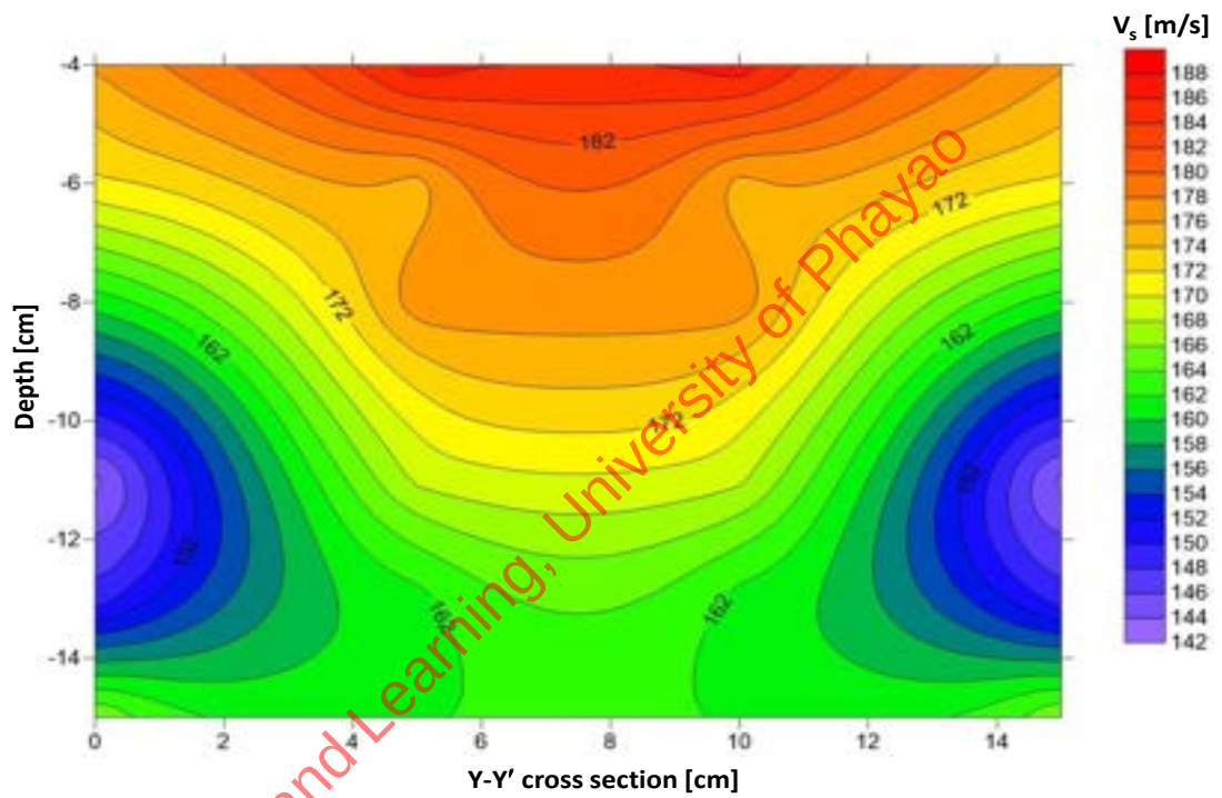
Figure 6-13 Contour of shear wave velocity for sample no.3 at cross section Y-Y' after Petcherdchoo et al. (2026).
