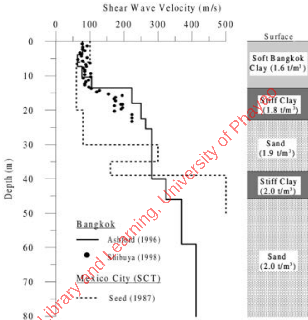
Figure 4-20 Generalized Bangkok soil and shear wave velocity profiles after Warnitchai et al. (2000).
