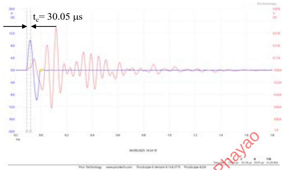
Figure 4-5 Calibration of bender element with a single period sinusoidal waveform.
