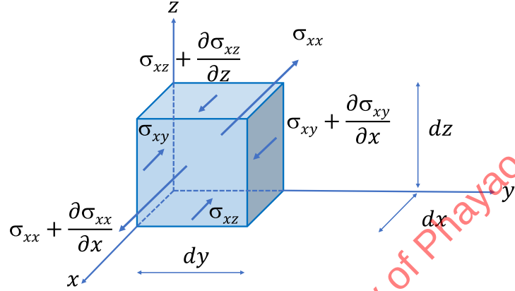
Figure 2-5 Stress along the x-axis acting upon a 3-D differential element.
