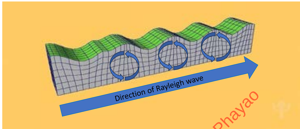
Figure 1-3 Rayleigh wave illustration.
