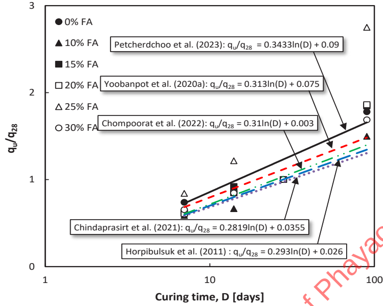
Figure 7-8 Relationships between q_u/q_{28} and curing time after Petcherdchoo et al. (2023).
