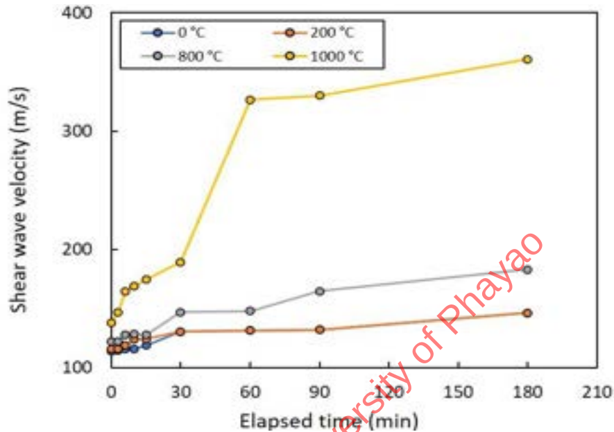
Figure 5-3. The shear wave velocity varied with elapsed time for thermal treatment after Iamchaturapatr et al. (2022b).
