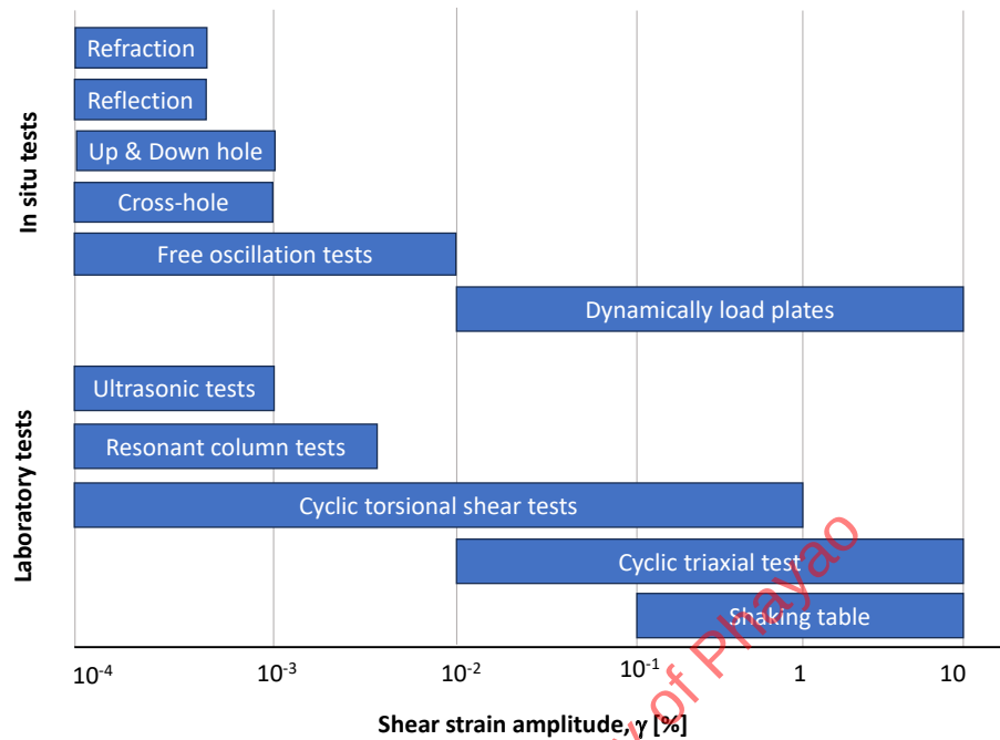
Figure 3-1 Overview of possible shear strain amplitudes after Studer et al. (2008).
