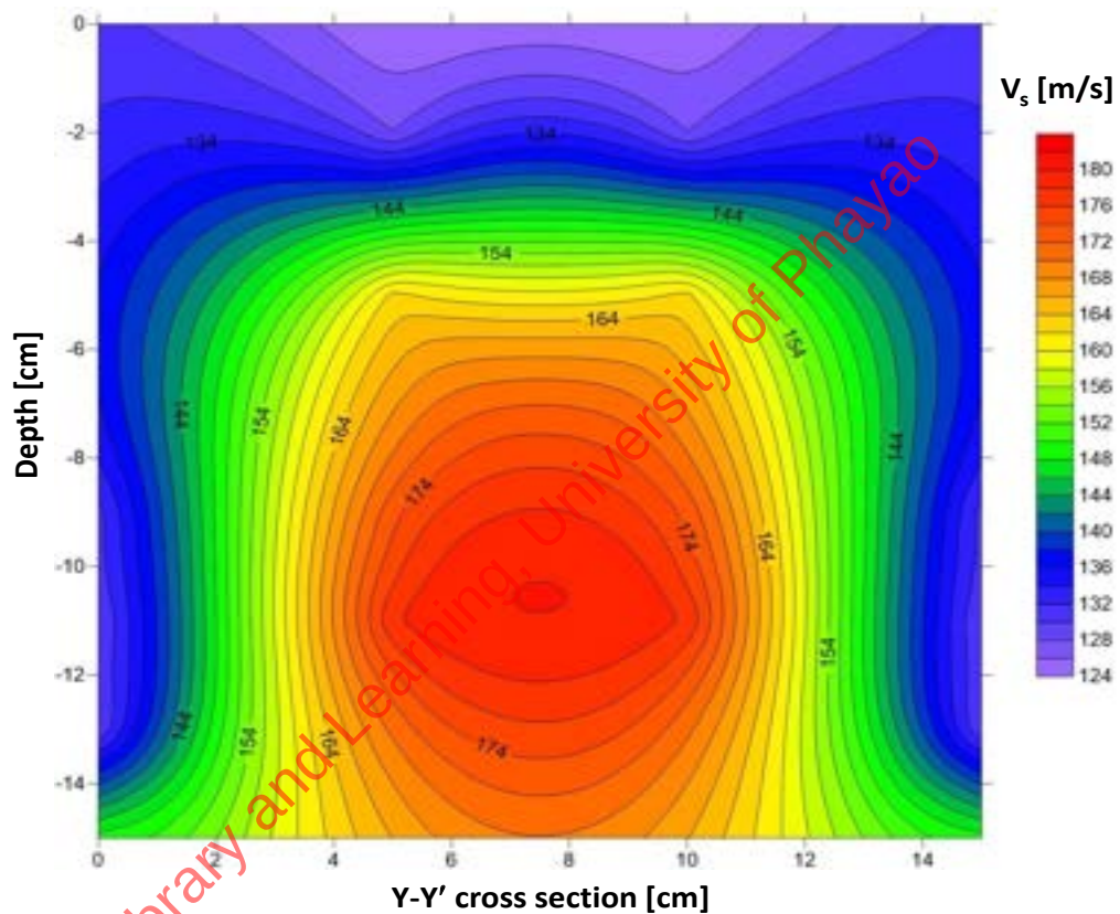
Figure 6-9 Contour of shear wave velocity for sample no.1 at cross section Y-Y' after Petcherdchoo et al. (2026).
