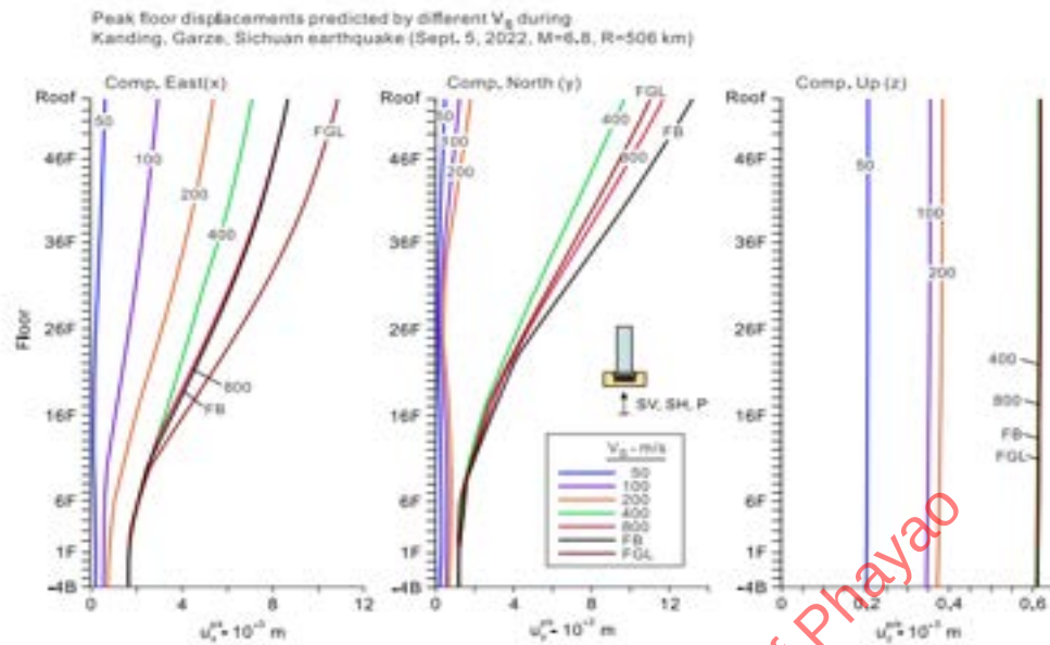
Figure 3-34 Peak floor displacements for different values of V_s during Kanding, Garze, Sichuan earthquake after Cruz et al. (2024).
