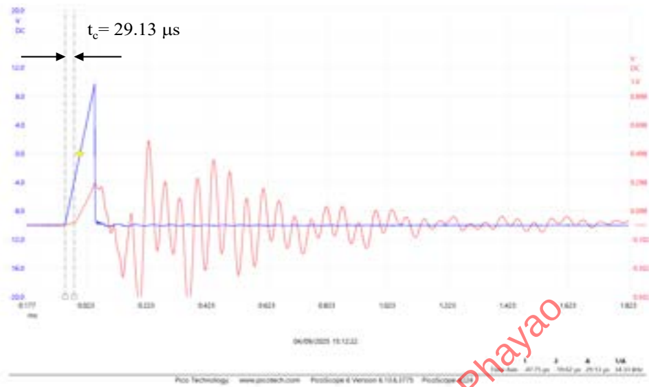
Figure 4-7 Calibration of bender element with a period triangle waveform.
