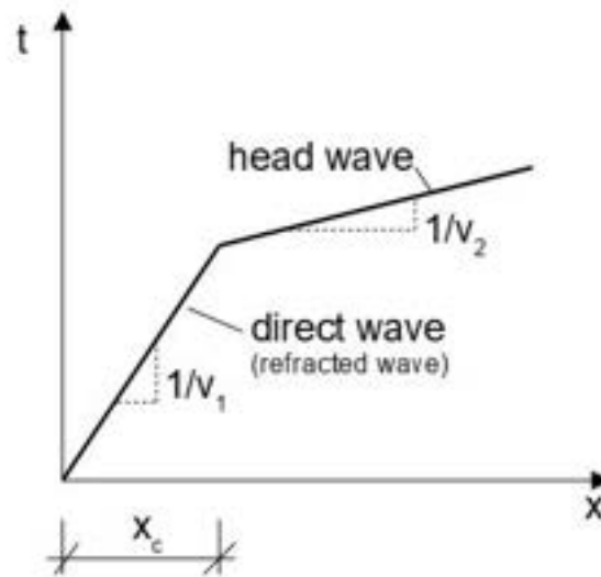
Figure 3-21 Time arrival diagram as result of a seismic refraction test after Kramer (1996).
